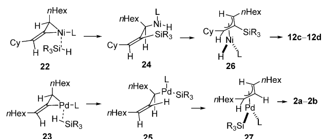
Figure 2. Proposed origin of the metal-directed regiodivergence.
